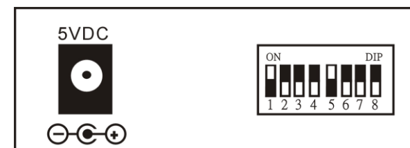
Figure 3. CVT-3512 Series Rear Panel
